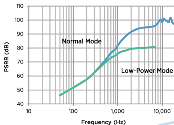
Figure 12: Typical PSRR
