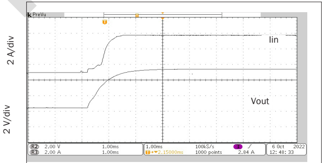
1 ms/div rMOR2805S INHIBIT RELEASE INRUSH CURRENT
