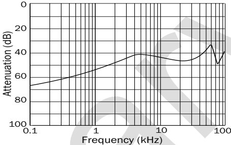
rMOR2805S Audio Rejection FIGURE 13
