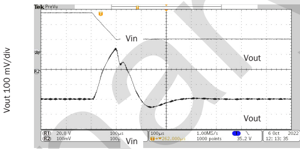
1 ms/div 50 to 15 V rMOR2805S STEP LINE RESPONSE
