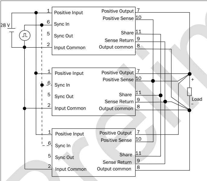
FIGURE 5: PARALLELING
