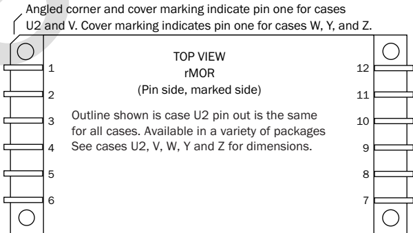
FIGURE 9: PIN OUT TOP VIEW
