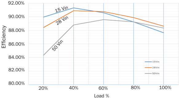
rMOR2805S Efficiency FIGURE 10
