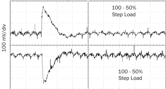
100 µs/div rMOR2805S STEP LOAD RESPONSE FIGURE 15
