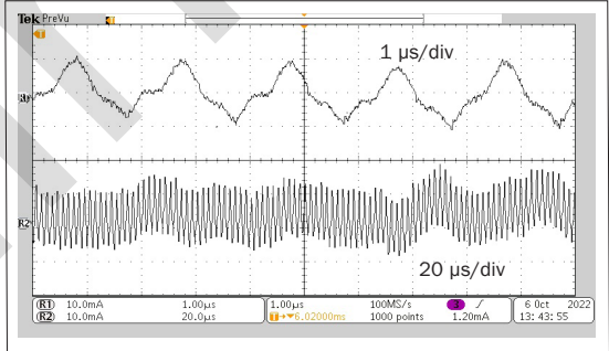
rMOR2805S Input Ripple Current (Iin) FIGURE 14
