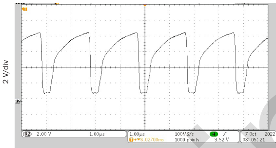
1 µs/div Sync Out Representative of all Models FIGURE 11
